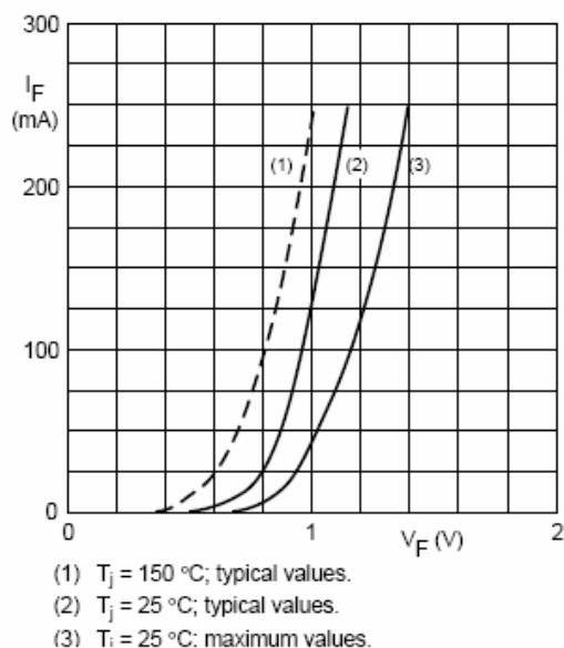
Fig.3 Forward current as a function of forward voltage.
