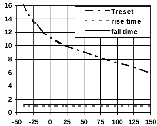
Figure 18 - Rise Time, Fall Time and Treset ( \mu\text{s} ) Vs T_j ( ^{\circ}\text{C} )
