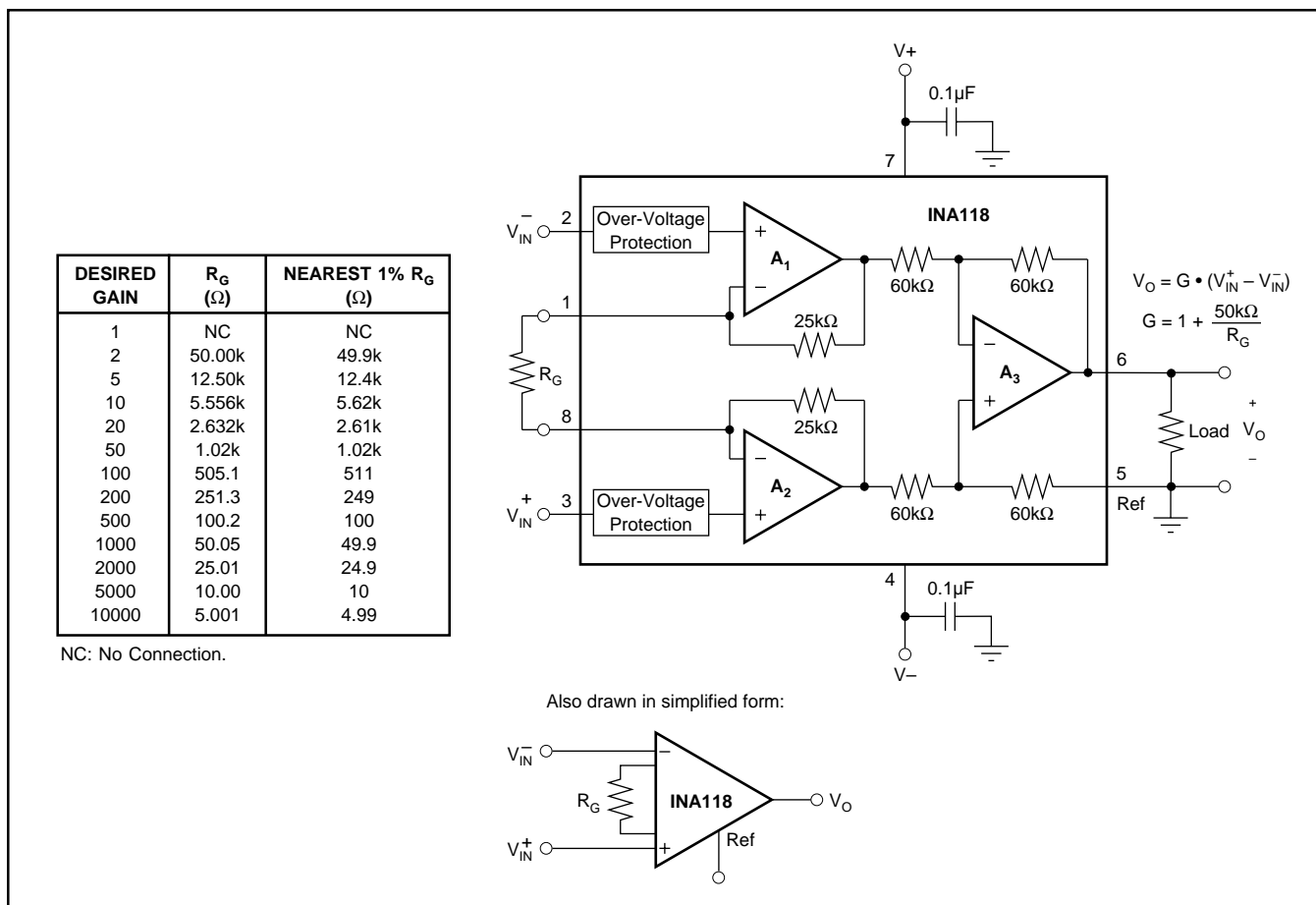
FIGURE 1. Basic Connections.
