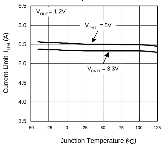
Current-Limit vs. Junction Temperature
