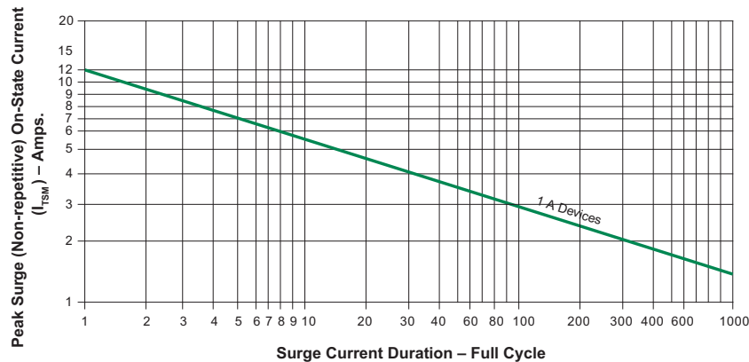
Figure 7: Surge Peak On-State Current vs. Number of Cycles
