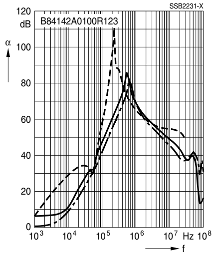
Filters for 100 A
