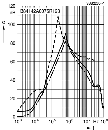
Filters for 75 A
