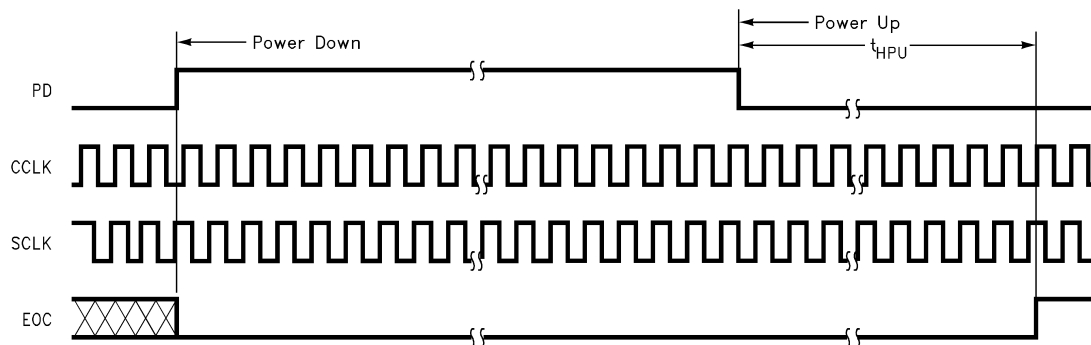
ADC12138 Hardware Power Up/Down
