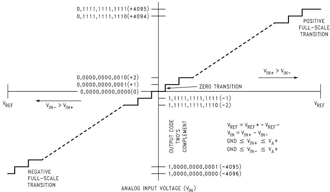
FIGURE 1. Transfer Characteristic
