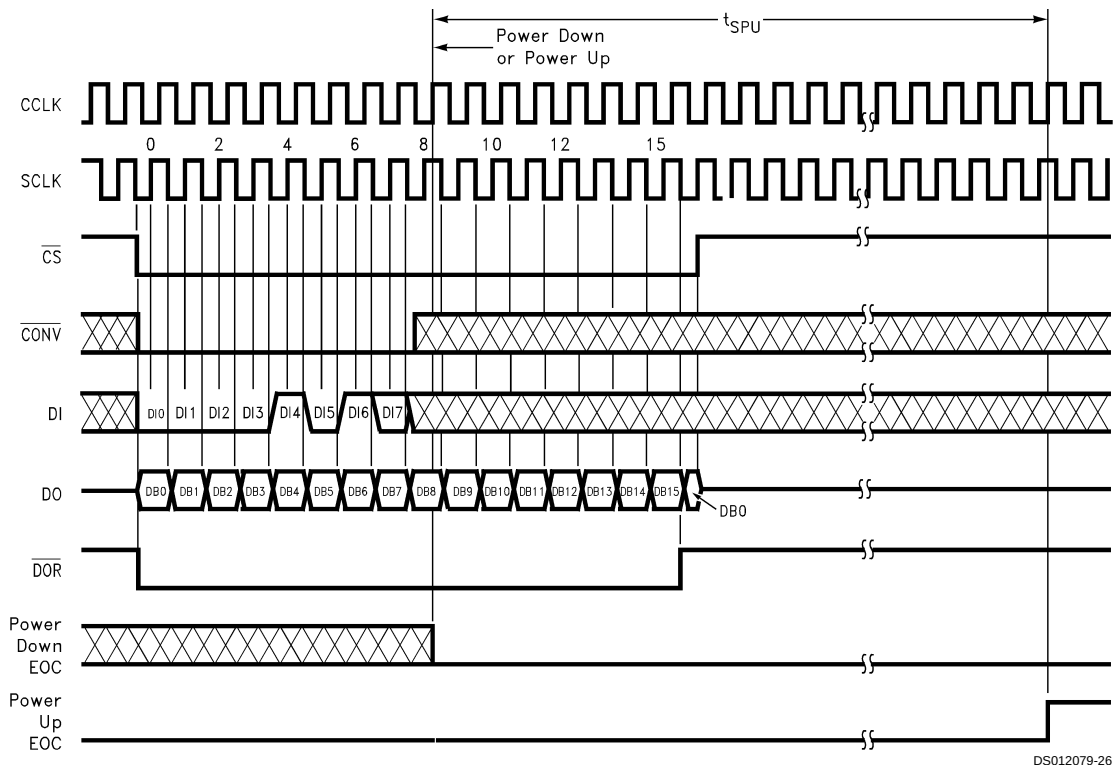
ADC12138 Software Power Up/Down Using \overline{\text{CS}} with 16-Bit Digital Output Format
