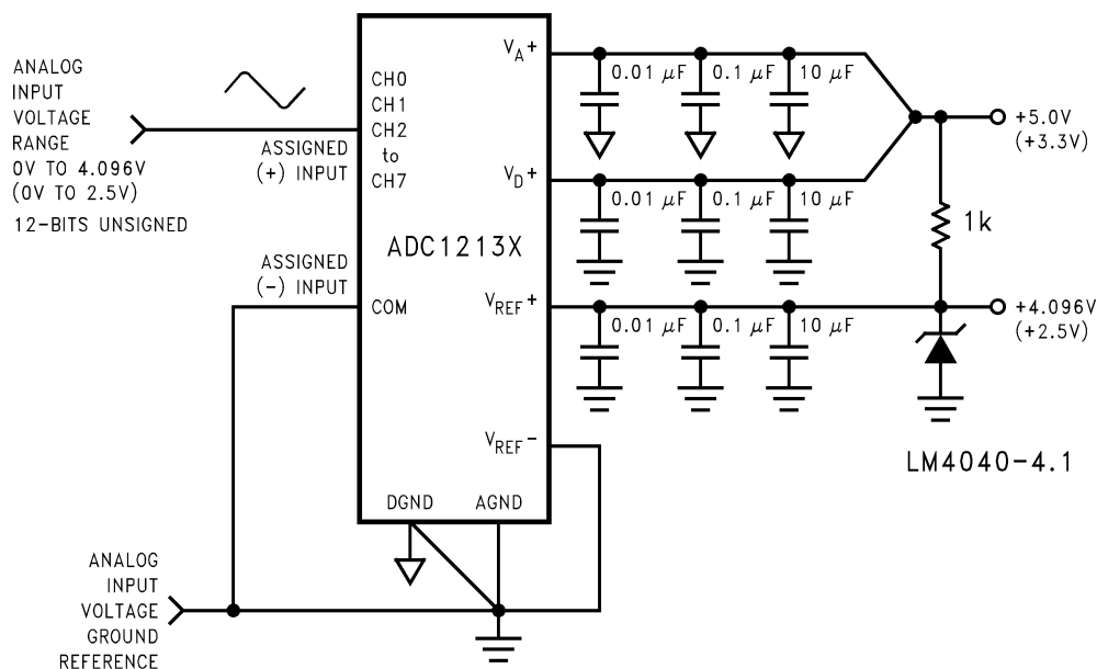
FIGURE 11. Single-Ended Biasing
