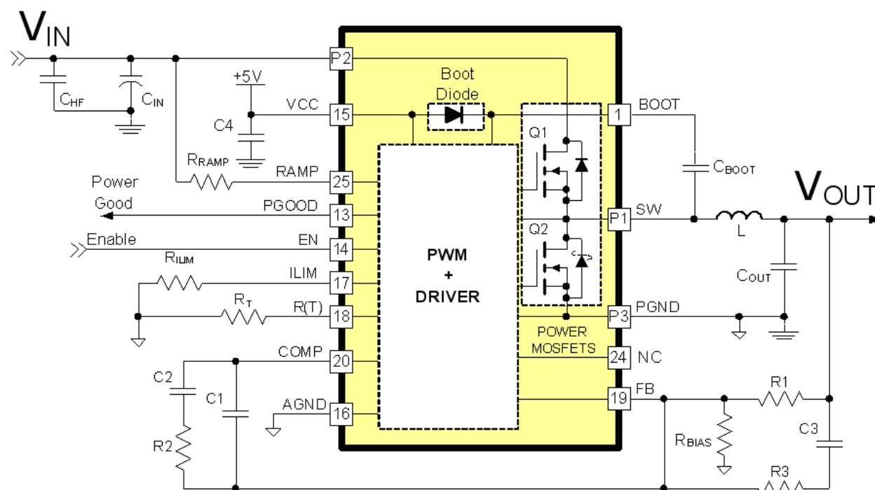
Figure 1. Typical Application
