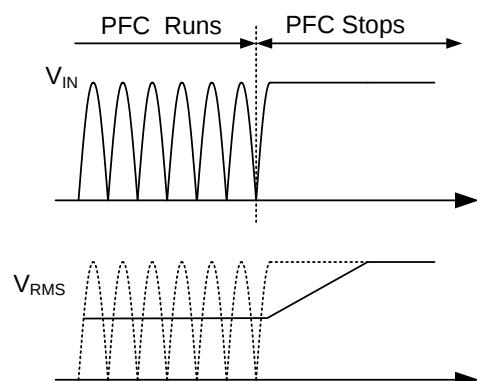
Figure 31. V_{RMS} According to the PFC Operation
