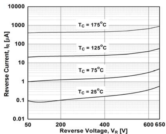
Figure 20. Reverse Current
