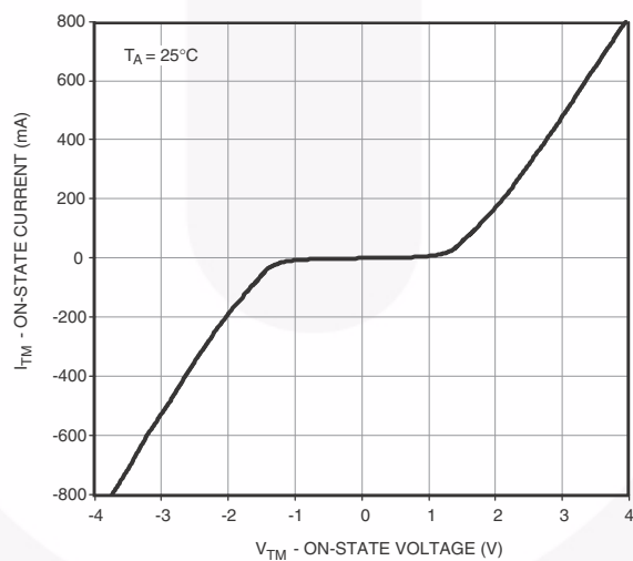
Fig. 9 On-State Characteristics
