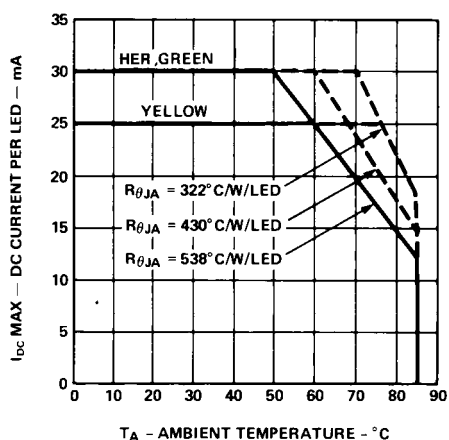
Figure 7. Maximum Allowable DC Current per LED vs. Ambient Temperature, T_J \text{ MAX} = 100^\circ\text{C} .
