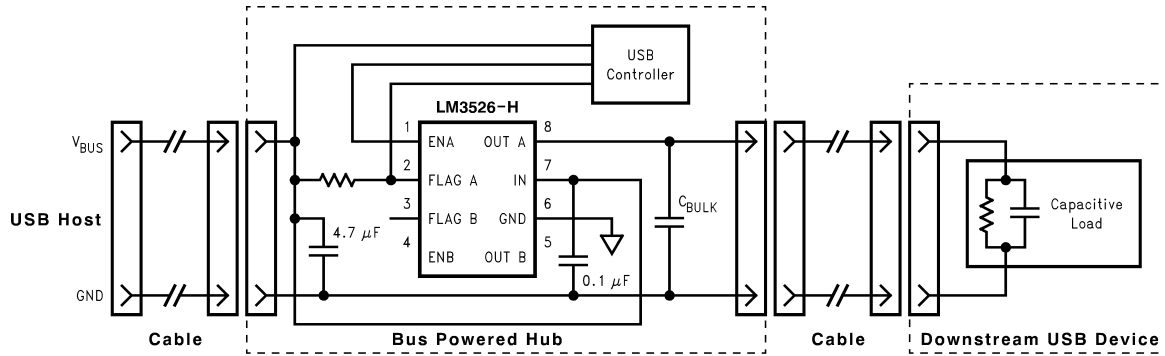
Figure 6. Soft-Start Application (Single port shown)
