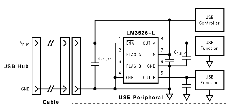
Figure 7. In-rush Current-limit Application
