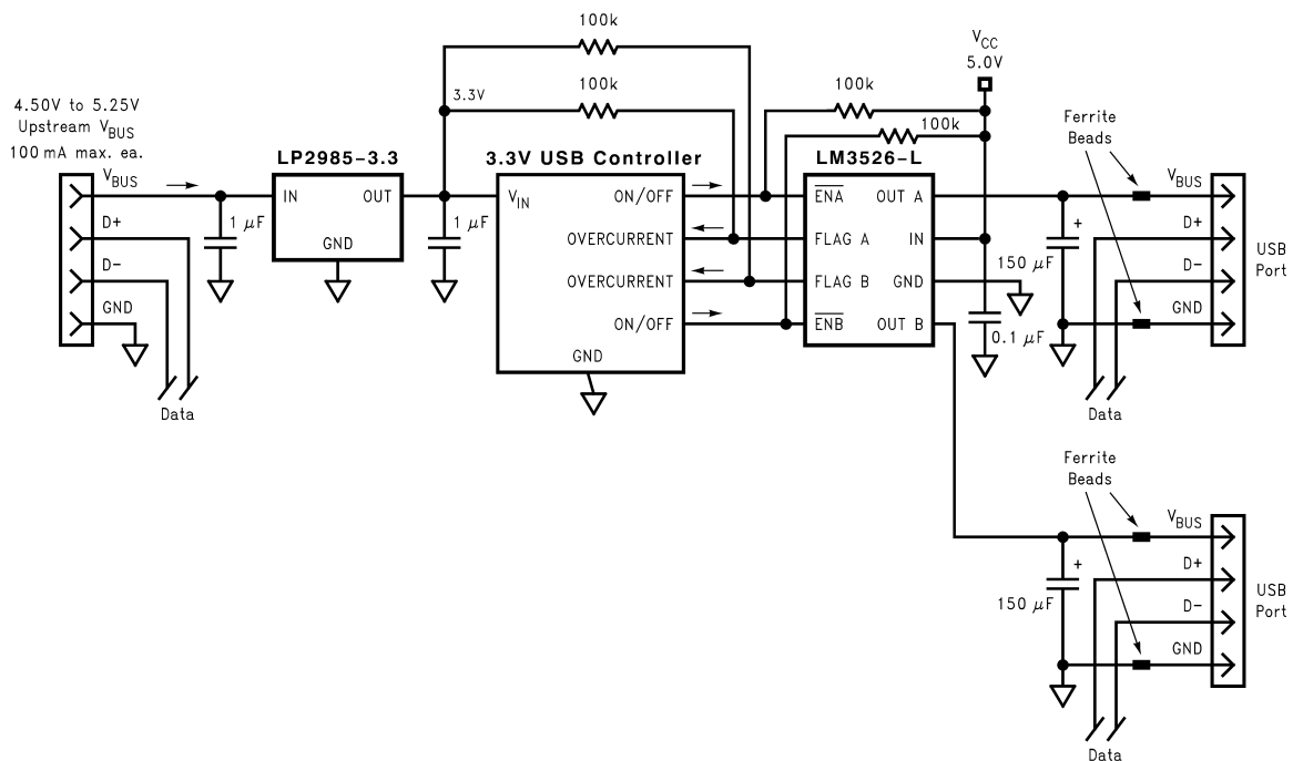
Figure 5. Dual-Port USB Self-Powered Hub
