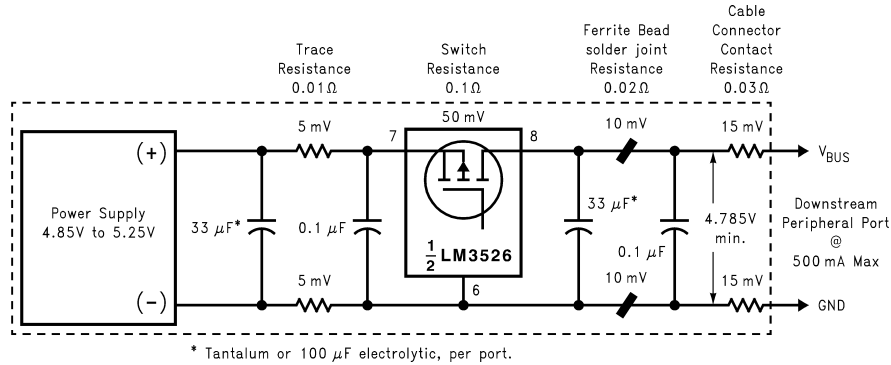
Figure 4. Self-Powered Hub Per-Port Voltage Drop
