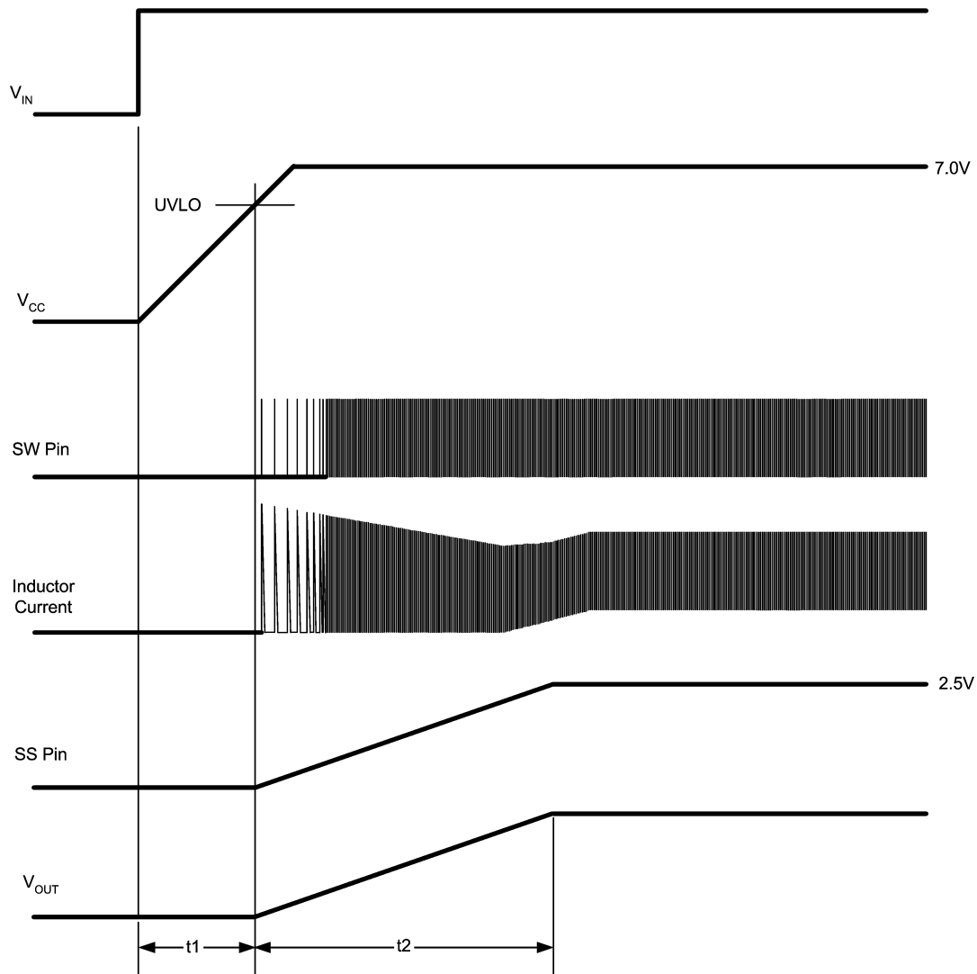
FIGURE 8. Startup Sequence
