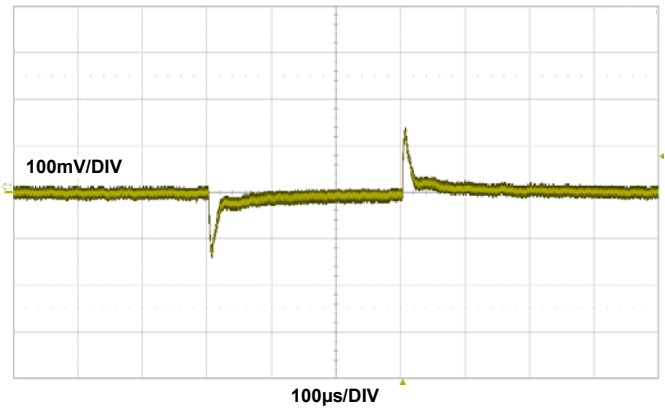
FIGURE 16. 1.5V OUT DUAL PHASE SINGLE OUTPUT TRANSIENT RESPONSE, I_{OUT} = 0A TO 20A , f_{SW} = 400kHz , C_{OUT} = 330\mu F POSCAP+ 10\mu F + 5 \times 100\mu F CERAMIC CAPACITOR
