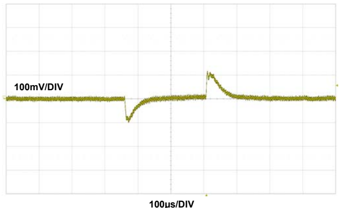
FIGURE 18. 1V OUT SIX PHASE SINGLE OUTPUT TRANSIENT RESPONSE, I_{OUT} = 0A TO 60A , f_{SW} = 350kHz , C_{OUT} = 6 \times 330\mu F POSCAP+ 7 \times 47\mu F + 6 \times 100\mu F CERAMIC CAPACITOR
