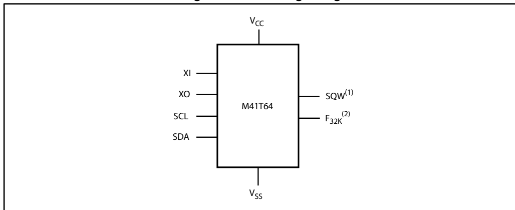
Figure 2: M41T64 logic diagram
