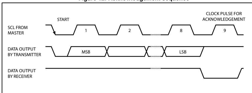
Figure 12: Acknowledgement sequence
