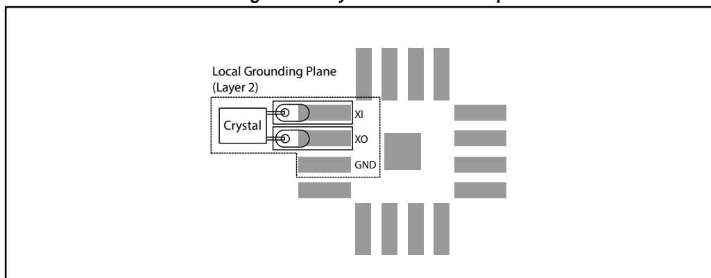
Figure 23: Crystal isolation example
