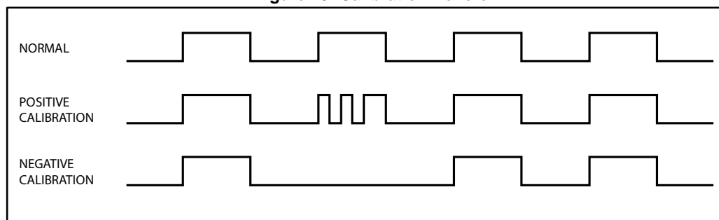
Figure 19: Calibration waveform
