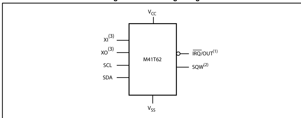
Figure 1: M41T62 logic diagram
