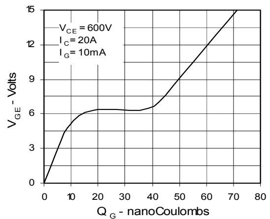
Fig. 10. Gate Charge
