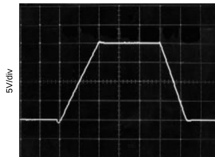
LARGE-SIGNAL STEP RESPONSE G = 1 , C_L = 300\text{pF}
