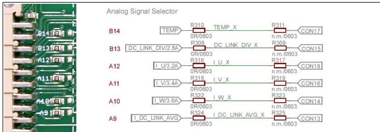
Figure 21 Analog Signal Selector
