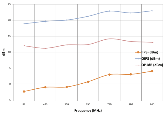
OP1dB, IIP3 and OIP3 over frequency (Vcc = Bref = 3.3V; Icc = 8mA)
