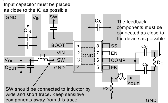
Figure 4. PCB Layout Guide
