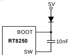
Figure 2. External Bootstrap Diode
