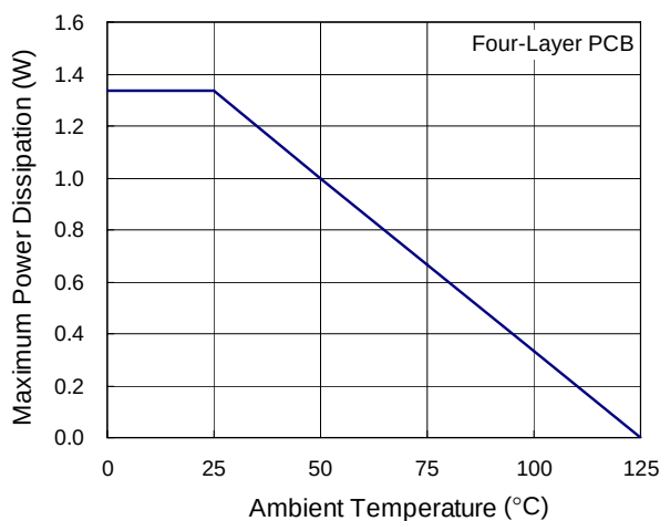
Figure 3. Derating Curve for RT8250 Package
