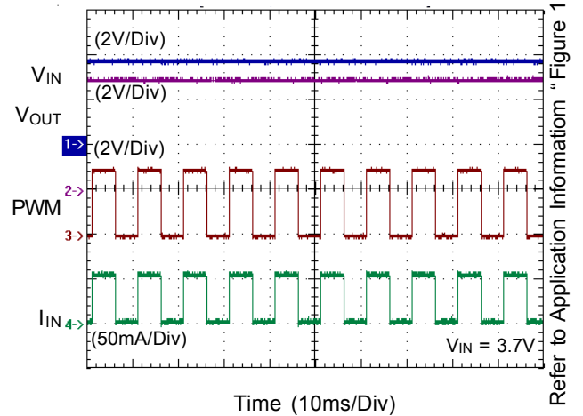
Dimming Operation
