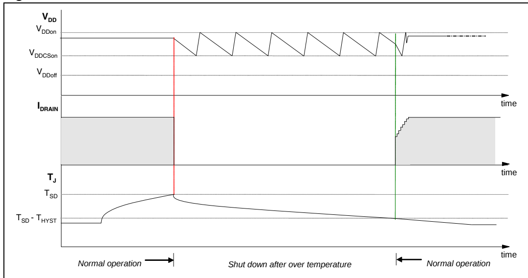
Figure 16. Thermal shutdown
