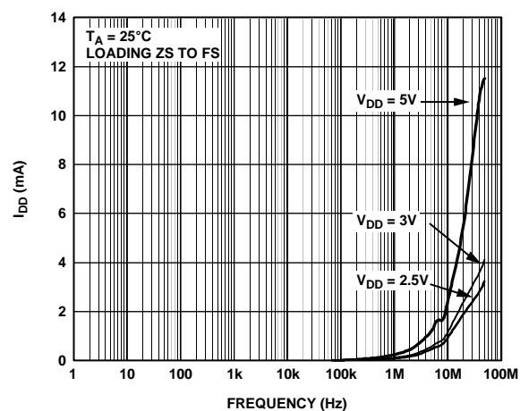
Figure 13. Supply Current vs. Update Rate
