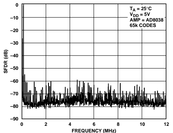
Figure 23. Wideband SFDR, f_{OUT} = 100 kHz, Clock = 25 MHz
