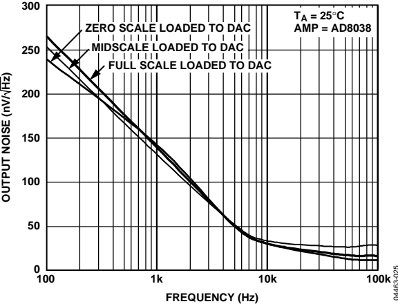
Figure 30. Output Noise Spectral Density
