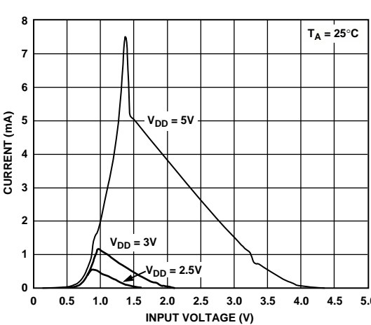
Figure 10. Supply Current vs. Logic Input Voltage
