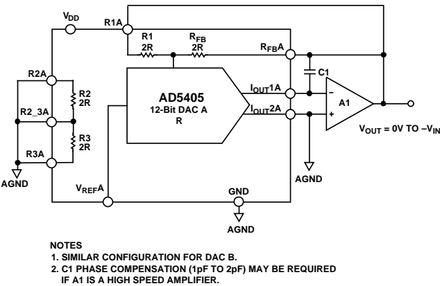
Figure 32. Unipolar Operation
