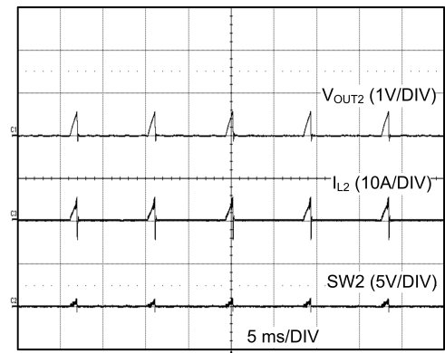
Switch Node Short Circuit Hiccup
