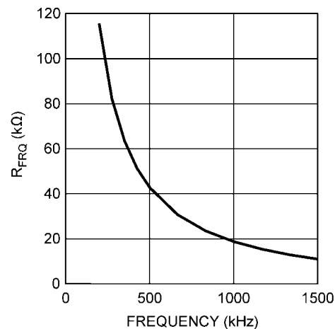
R_{FRQ} vs Switching Frequency
