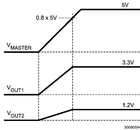
FIGURE 5. Tracking a Master Supply with Equal Start Time
