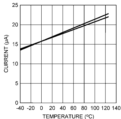
Enable Current Threshold vs Temperature
