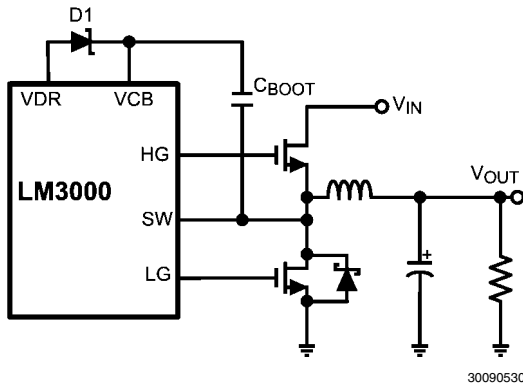
FIGURE 9. Bootstrap Circuit
