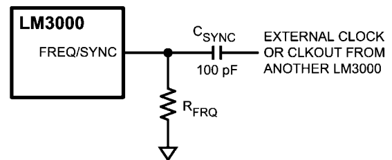
FIGURE 8. Clock Synchronization Circuit
