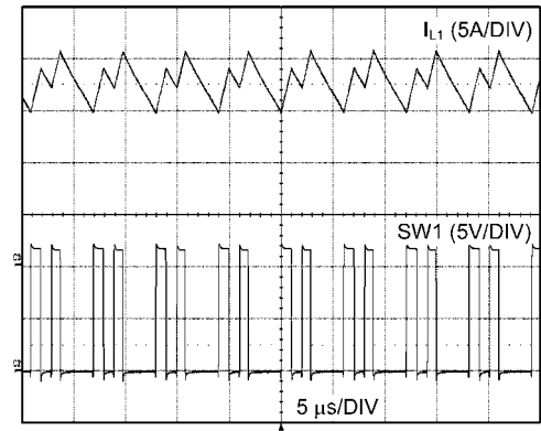
Pulse Skipping during Over-Current Condition
