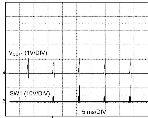
Output Short Circuit Hiccup
