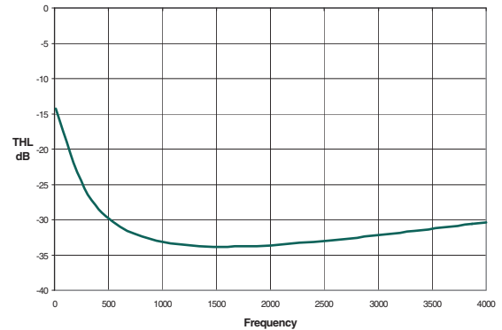
Figure 10. Transhybrid Loss
