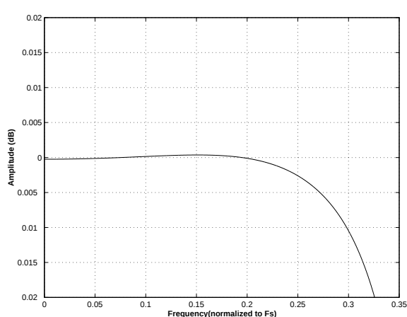
Figure 37. Double-Speed (slow) Passband Ripple
