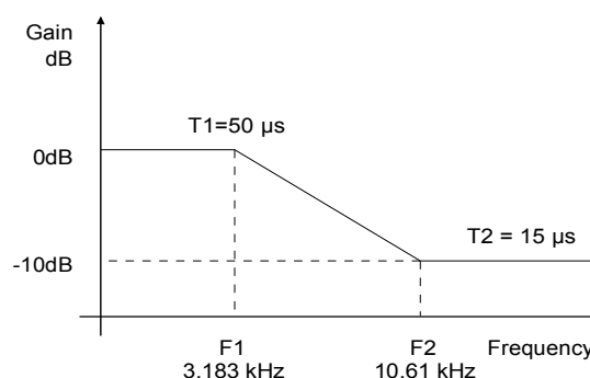
Figure 18. De-Emphasis Curve
