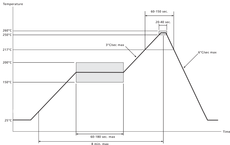
Figure 7-1: Maximum Pb-free Solder Reflow Profile
