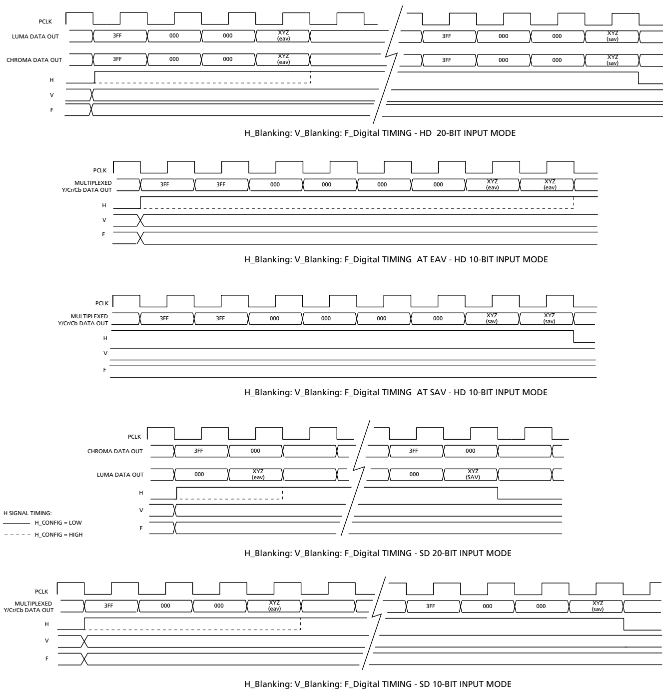
Figure 4-2: H_Blanking, V_Blanking, F_Digital Timing
