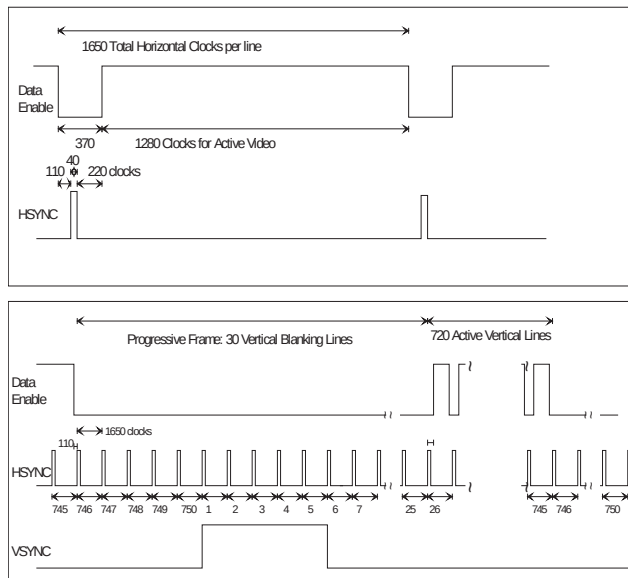
Figure 4-6: HSYNC:VSYNC:DE Input Timing 1280 x 720p @ 50
