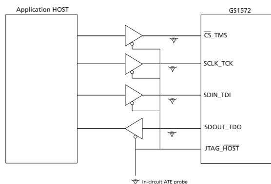
Figure 4-15: In-Circuit JTAG
