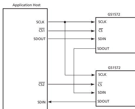
Figure 4-10: Gennum Serial Peripheral Interface (GSPI)
