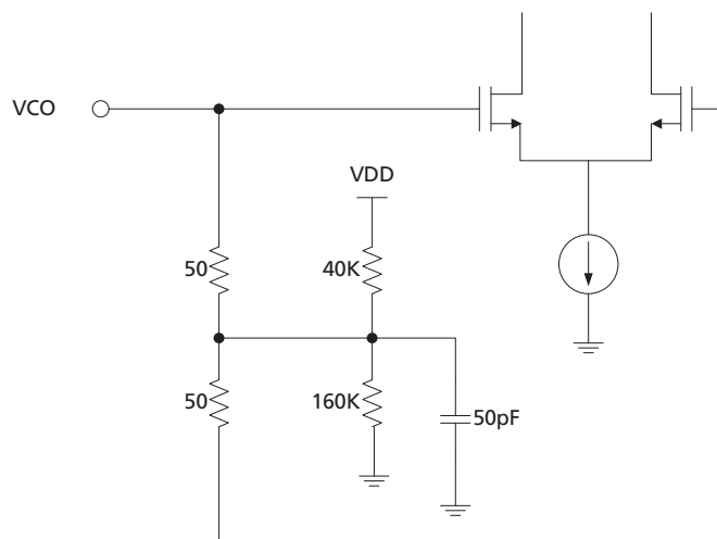
Figure 3-4: VCO Input
