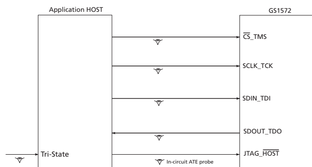
Figure 4-16: System JTAG
