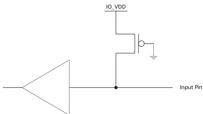
Figure 3-5: Digital Input Pin with Weak Pull Up(>33k \Omega ) (PCLK, DIN[19:0])
