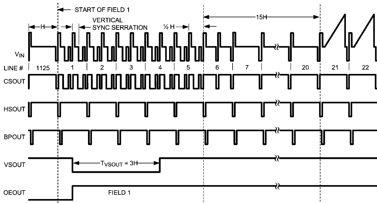
FIGURE 7. 1080I Field 1 Vertical Interval
