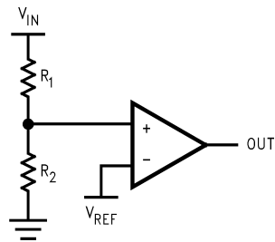
FIGURE 4. Threshold Detector
