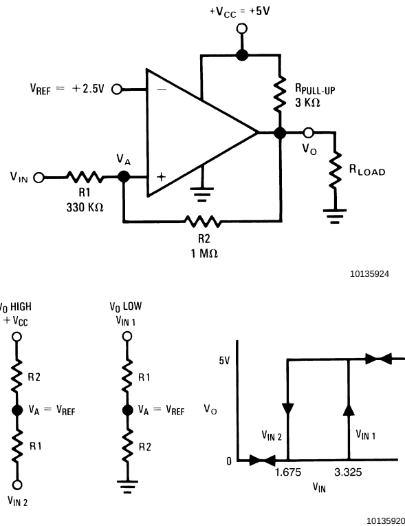
FIGURE 2. Non-Inverting Comparator with Hysteresis
