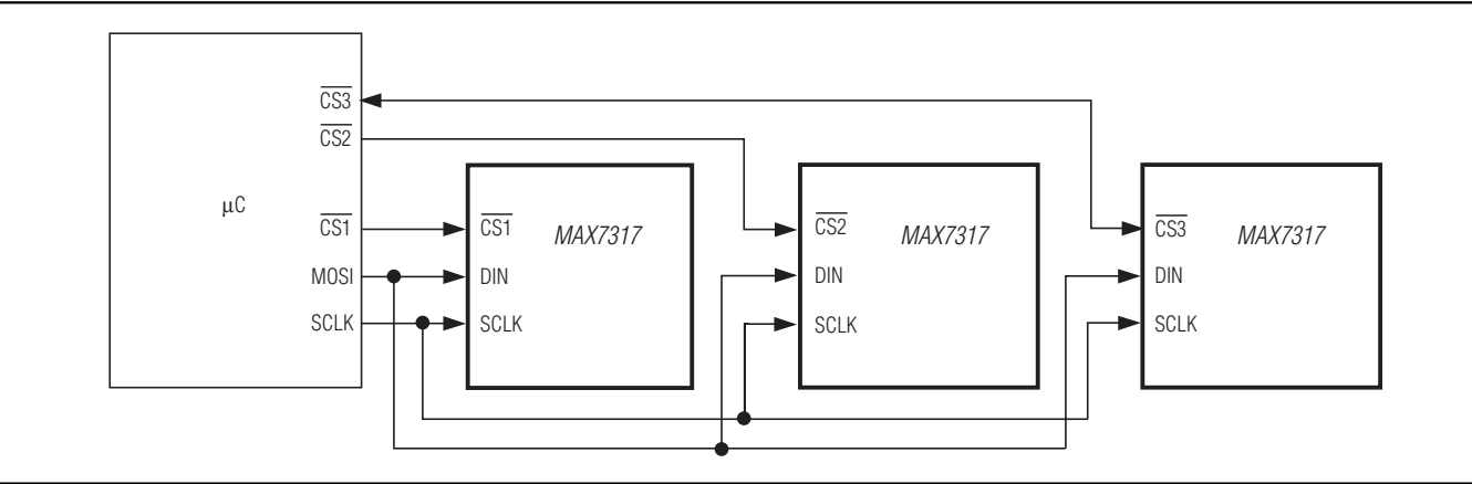
Figure 2. MAX7317 Multiple CS Connection
