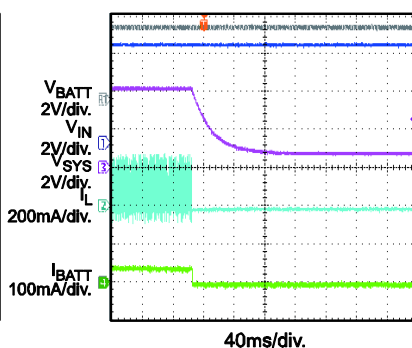
Thermal Shutdown
