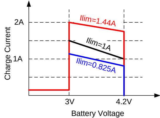
Figure 7— I_{CHG} Variation with Different Input Current Limit
