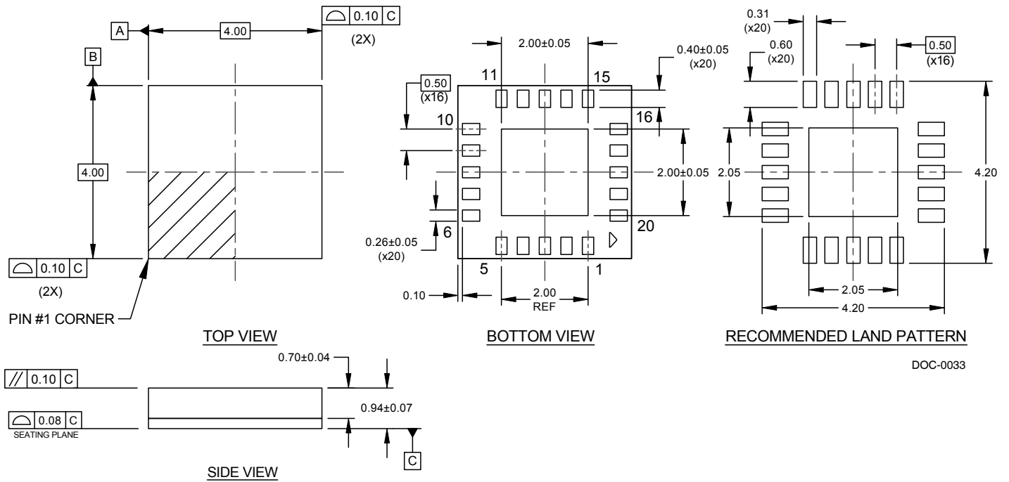
Figure 21. Package Drawing 20-lead 4 × 4 mm LGA
