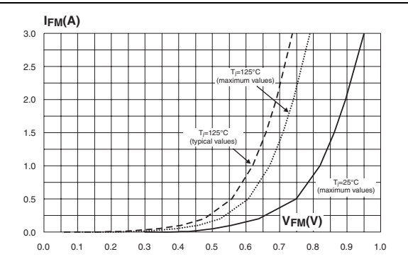
Figure 9. Forward voltage drop versus forward current (all packages)
