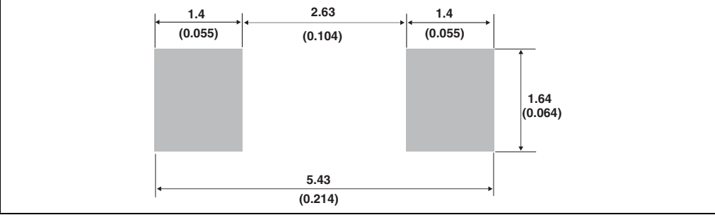
Figure 11. Footprint (dimensions in mm)
