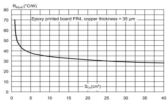
Figure 14: Thermal resistance junction to ambient versus copper surface under tab (D²PAK)
