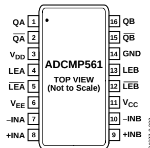
Figure 2. ADCMP561 16-Lead QSOP
