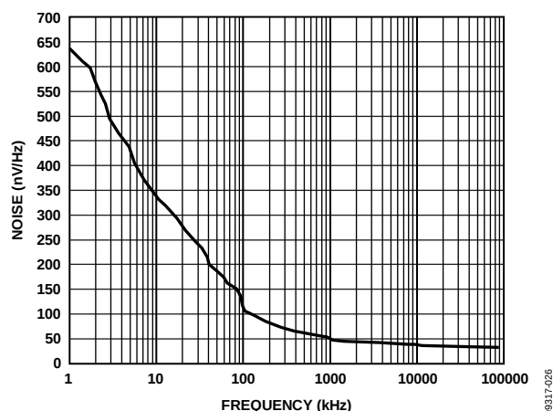
Figure 29. ADV3225 Output Noise Density, 100 Ω Load
