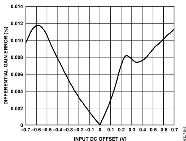
Figure 48. ADV3225 Differential Gain Error
