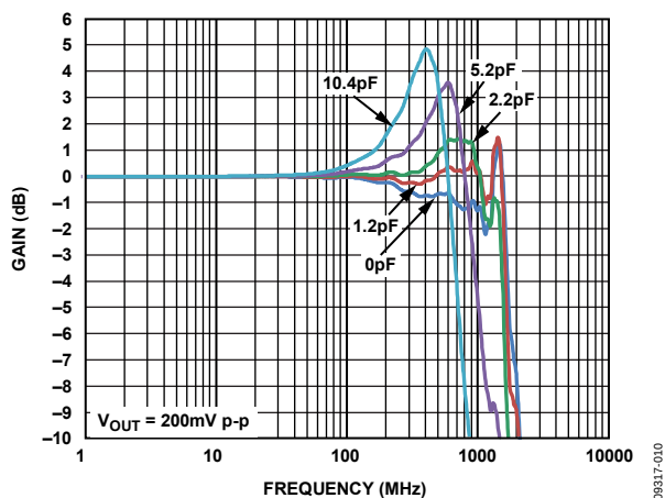
Figure 9. ADV3224 Small Signal Frequency Response with Capacitive Loads
