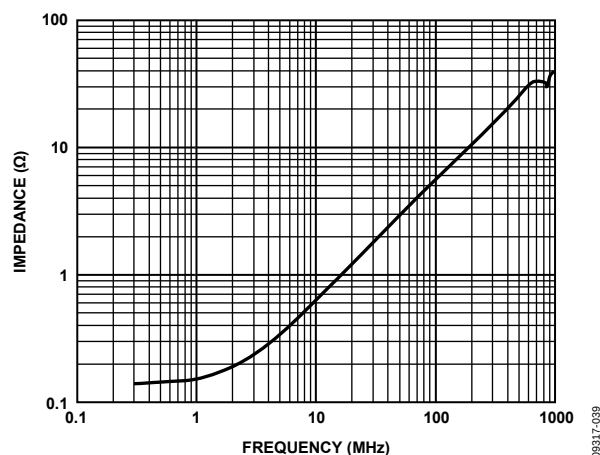
Figure 41. ADV3225 Output Impedance, Enabled
