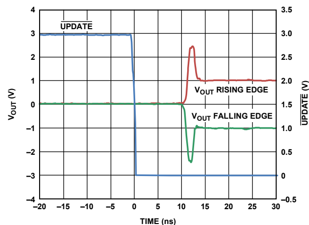
Figure 44. ADV3224 Enable Time
