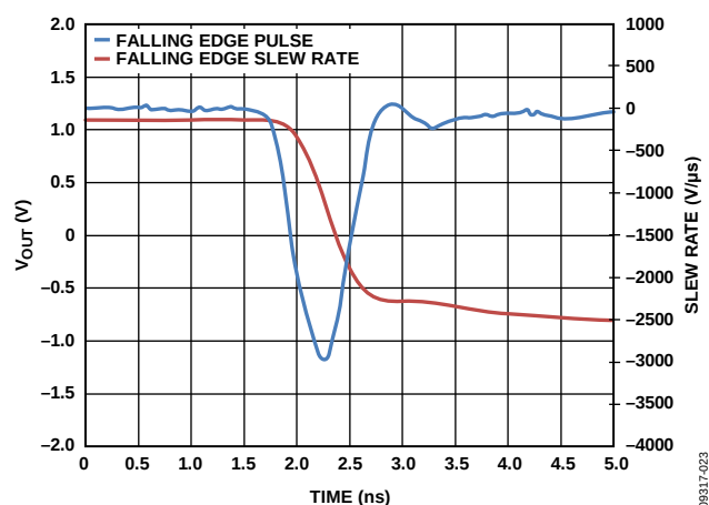
Figure 23. ADV3225 Falling Edge Slew Rate
