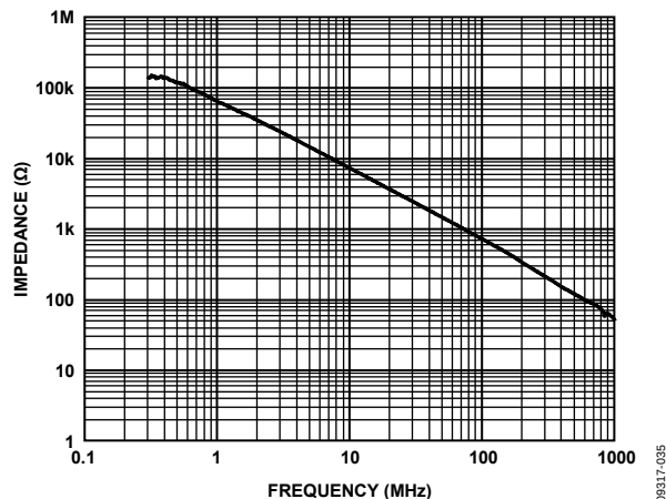
Figure 37. ADV3224 Output Impedance, Disabled
