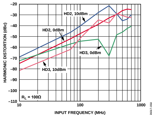
Figure 57. ADV3225 Harmonic Distortion, 100 \Omega Load
