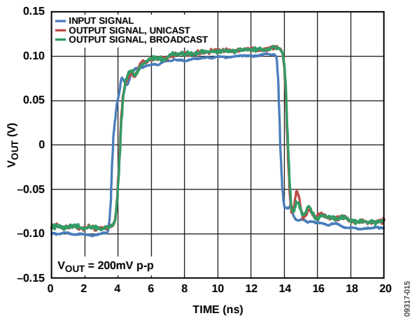
Figure 14. ADV3224 Small Signal Pulse Response
