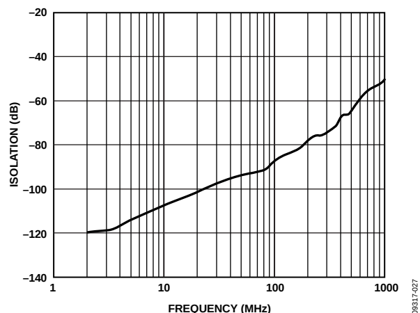
Figure 30. ADV3225 Off Isolation
