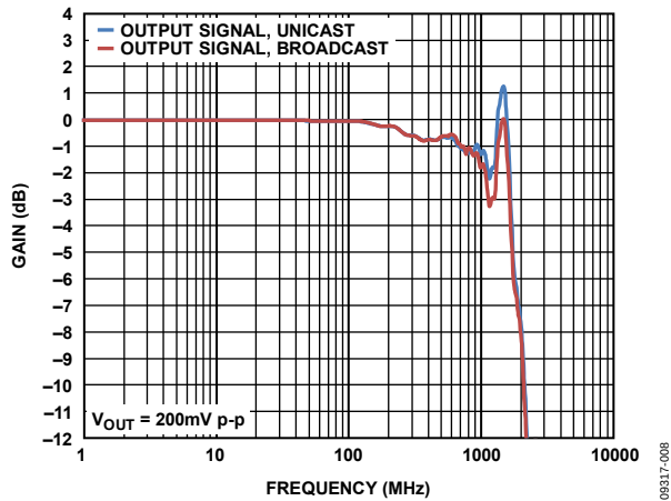
Figure 7. ADV3224 Small Signal Frequency Response
