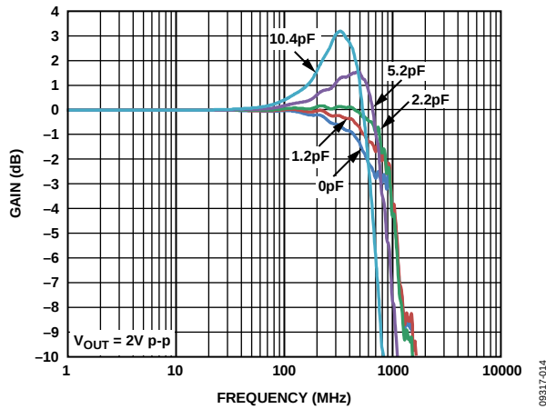
Figure 13. ADV3224 Large Signal Frequency Response with Capacitive Loads
