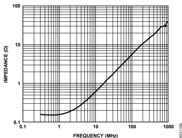
Figure 38. ADV3224 Output Impedance, Enabled
