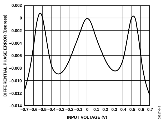
Figure 52. ADV3225 Differential Phase Error
