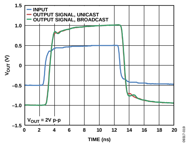
Figure 18. ADV3225 Large Signal Pulse Response
