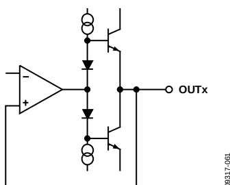
Figure 59. Analog Output Enabled
