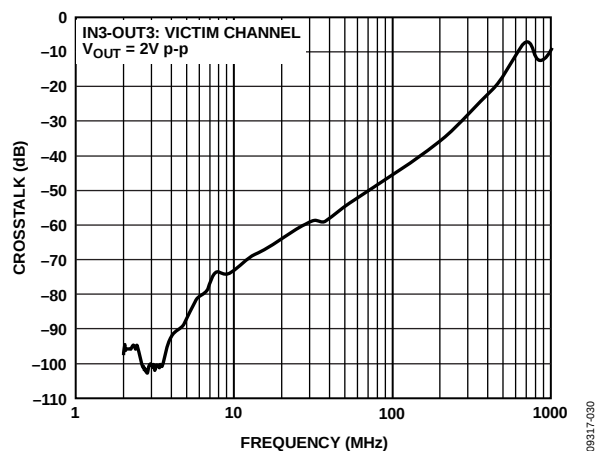
Figure 32. ADV3224 Crosstalk, All Hostile, RTO
