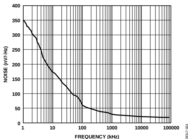
Figure 26. ADV3224 Output Noise Density, 100 Ω Load
