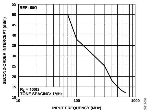
Figure 55. ADV3225 Output Second-Order Intercept, 100 \Omega Load
