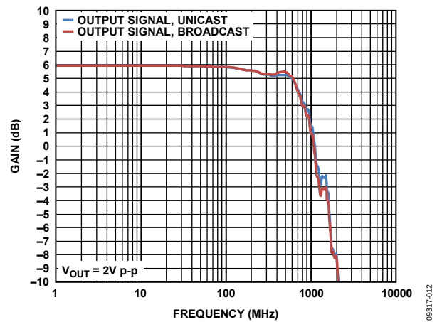
Figure 11. ADV3225 Large Signal Frequency Response
