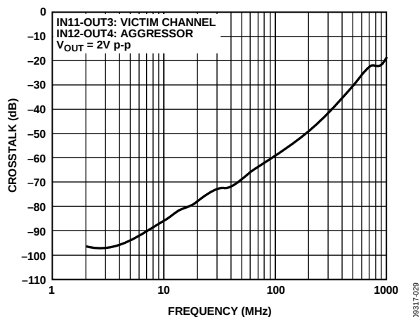
Figure 31. ADV3224 Crosstalk, One Adjacent Channel, RTO
