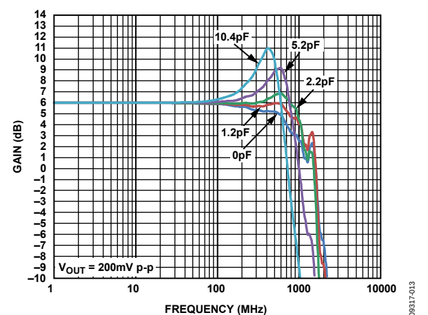
Figure 12. ADV3225 Small Signal Frequency Response with Capacitive Loads
