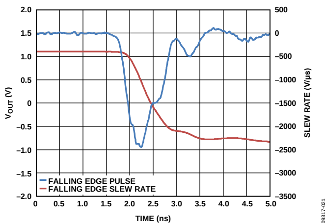
Figure 20. ADV3224 Falling Edge Slew Rate
