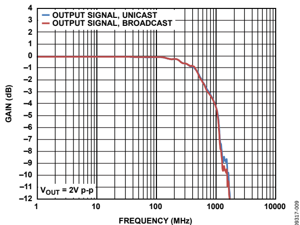
Figure 8. ADV3224 Large Signal Frequency Response
