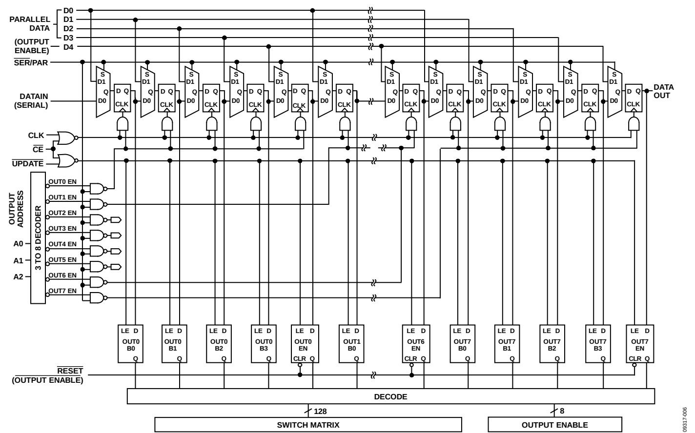
Figure 6. Logic Diagram
