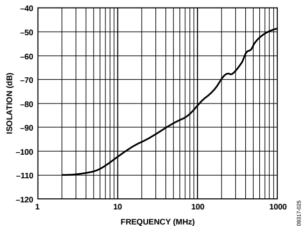
Figure 27. ADV3224 Off Isolation
