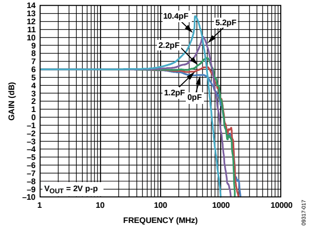
Figure 16. ADV3225 Large Signal Frequency Response with Capacitive Loads
