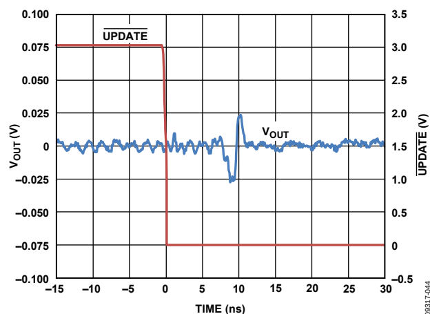
Figure 46. ADV3225 Switching Glitch
