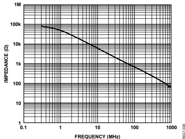
Figure 40. ADV3225 Output Impedance, Disabled
