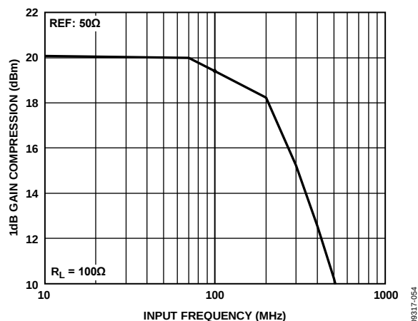
Figure 51. ADV3225 1 dB Gain Compression, 100 \Omega Load
