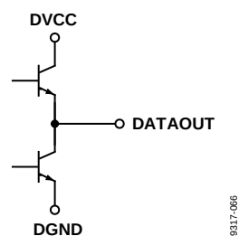
Figure 64. Logic Output
