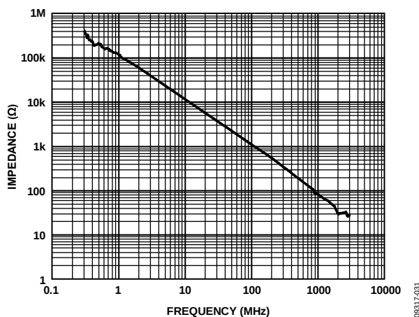
Figure 33. ADV3224 Input Impedance
