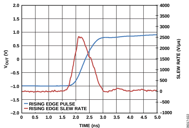
Figure 22. ADV3225 Rising Edge Slew Rate
