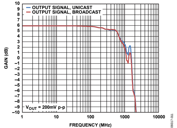
Figure 10. ADV3225 Small Signal Frequency Response
