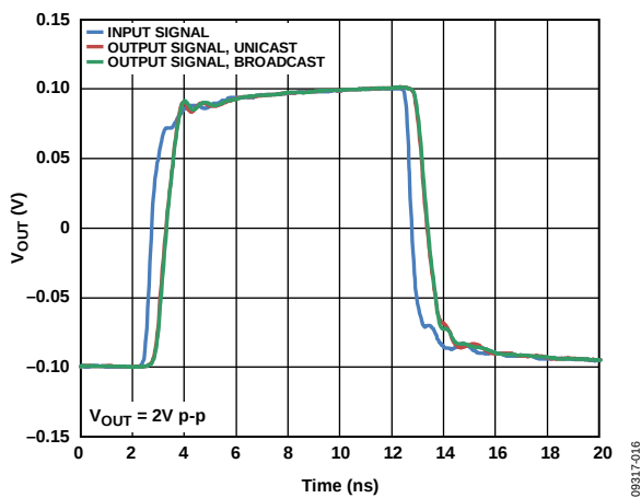
Figure 15. ADV3224 Large Signal Pulse Response
