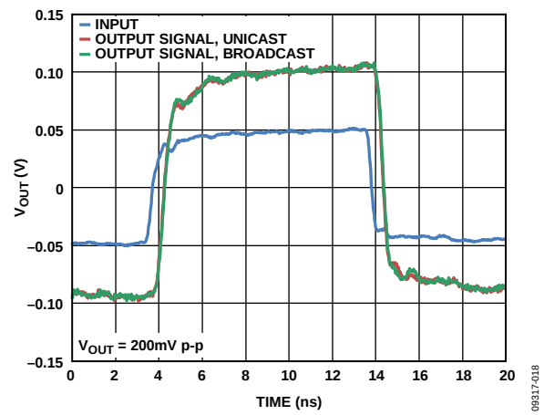
Figure 17. ADV3225 Small Signal Pulse Response
