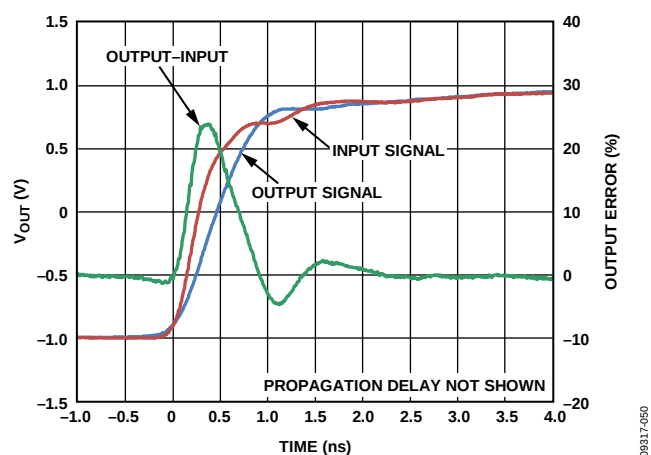
Figure 24. ADV3225 Settling Time
