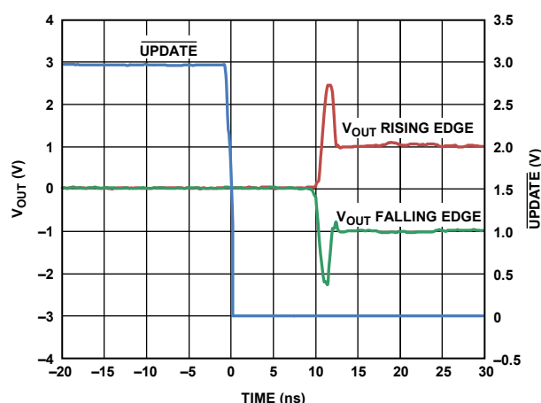
Figure 47. ADV3225 Enable Time
