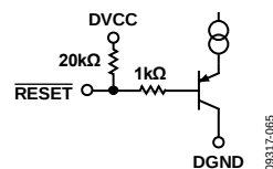
Figure 63. Reset Input
