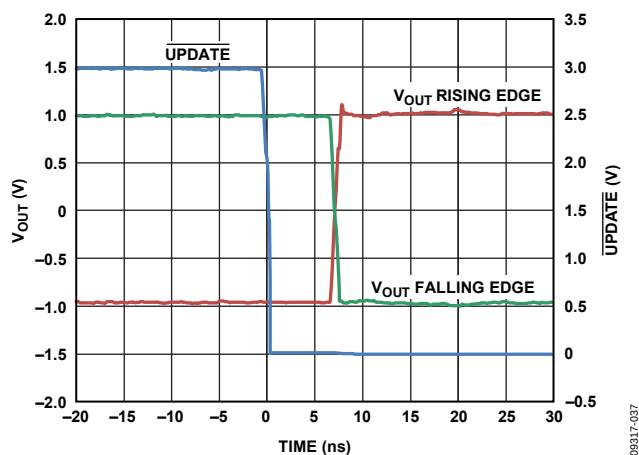
Figure 39. ADV3224 Switching Time
