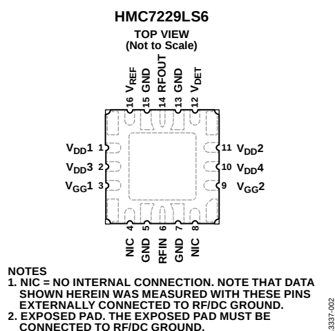
Figure 2. Pin Configuration
