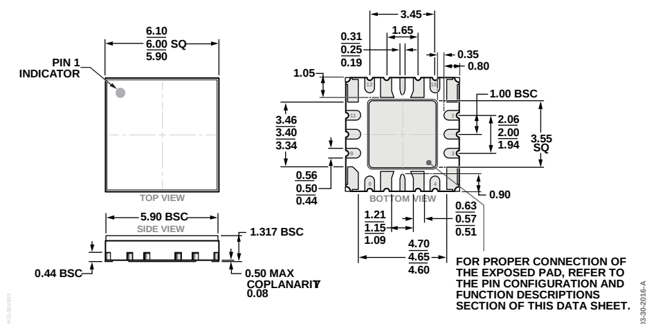
Figure 36. 16-Terminal Ceramic Leadless Chip with Heat Sink [LCC_HS] (EP-16-2)
