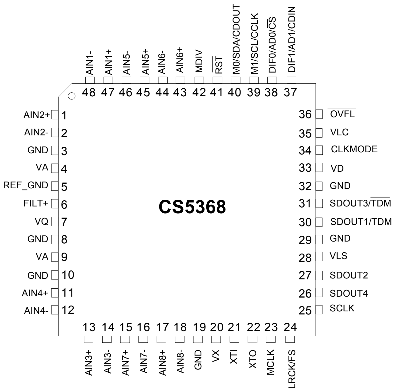
Figure 1. CS5368 Pinout
