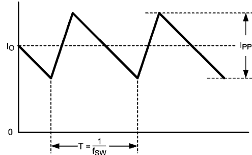
FIGURE 6. Inductor Current
