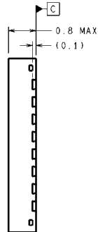
32 Pin LLP NS Package Number SQA32A
