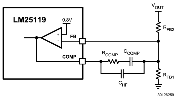
FIGURE 7. Feedback Configuration
