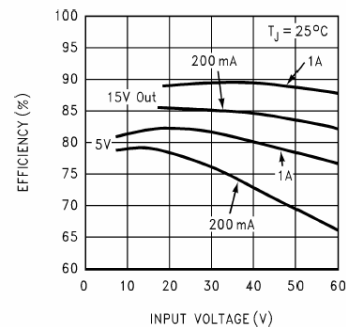
Efficiency
