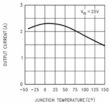
Current Limit
