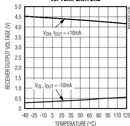
RECEIVER OUTPUT VOLTAGE vs. TEMPERATURE
