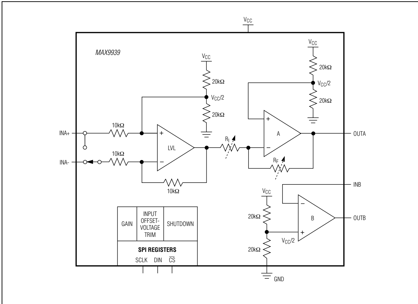
Functional Diagram
