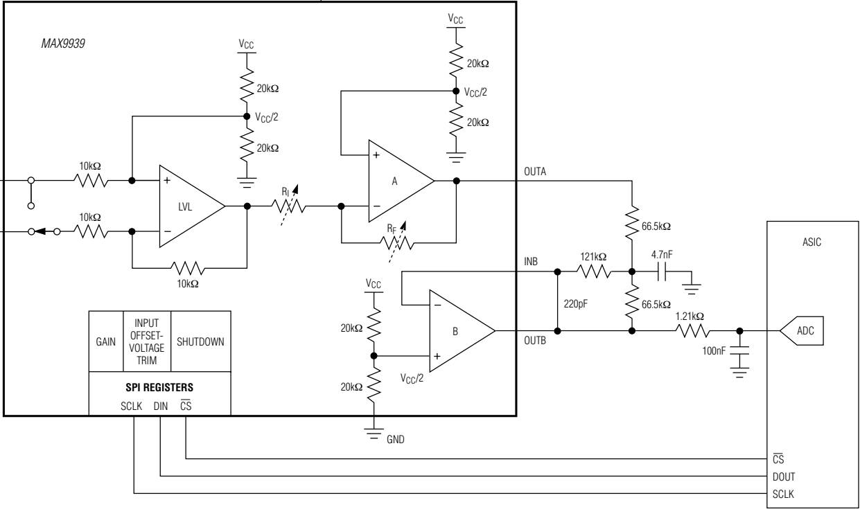
Figure 3. Using the MAX9939 Output Amplifier as an Anti-Aliasing Filter (Corner Frequency = 1.3kHz) to Maximize Nyquist Bandwidth
