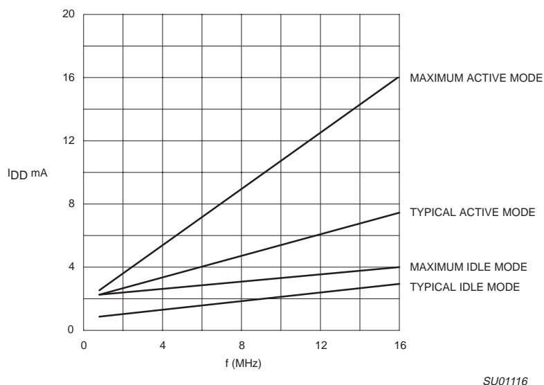
Figure 56. 16MHz Version Supply Current ( I_{DD} ) as a Function of Frequency at XTAL1 ( f_{OSC} )
