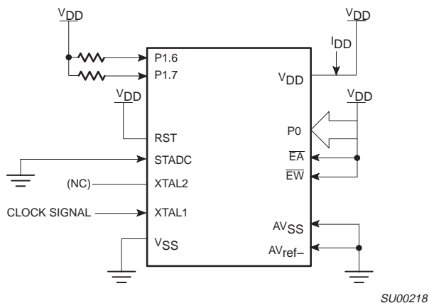
Figure 57. I_{DD} Test Condition, Active Mode All other pins are disconnected 1
