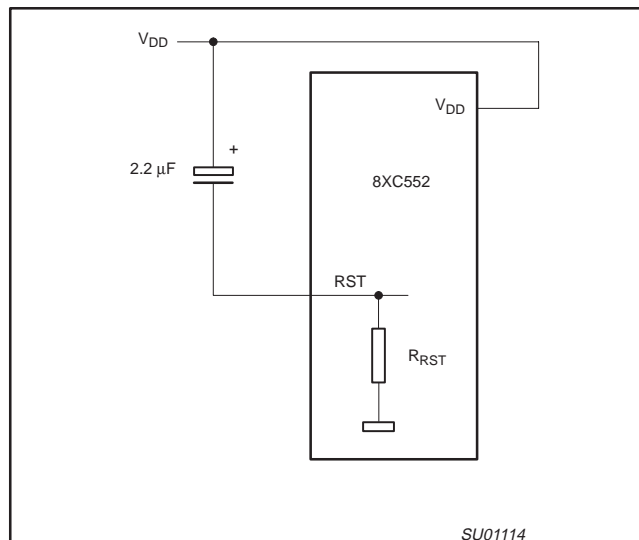
Figure 2. Power-On Reset
