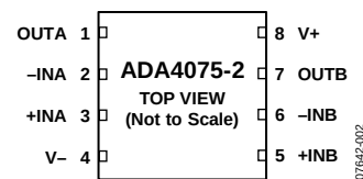
Figure 2. 8-Lead, 2 mm × 2 mm LFCSP
