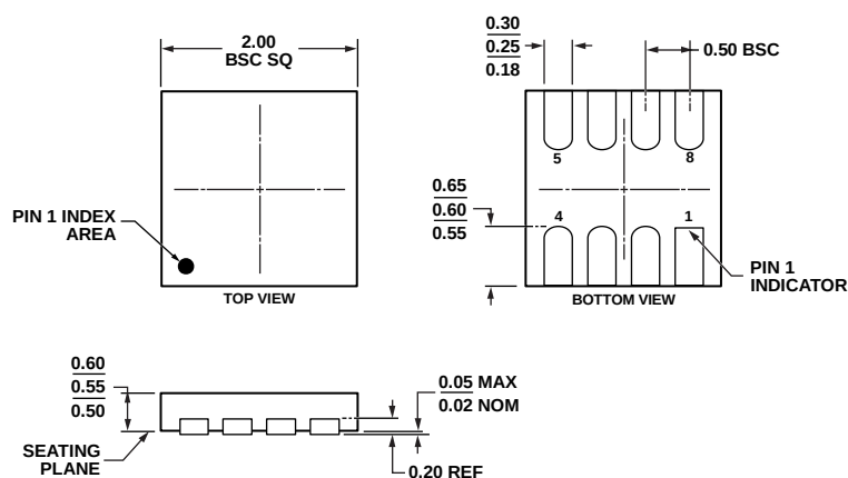
Figure 72. 8-Lead Lead Frame Chip Scale Package [LFCSP_WD] 2 mm x 2 mm Body, Very Very Thin, Dual Lead (CP-8-6)
