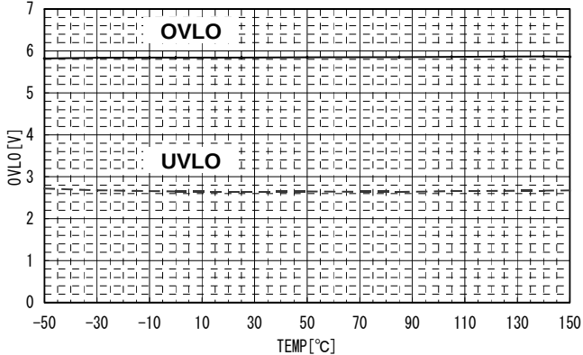
Fig. 10 UVLO/OVLO vs. Temperature
