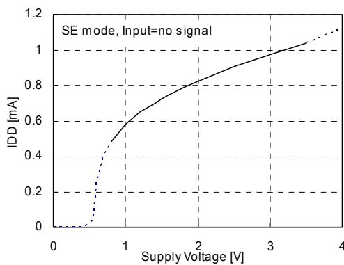
Fig. 30 IDD vs. Supply Voltage
