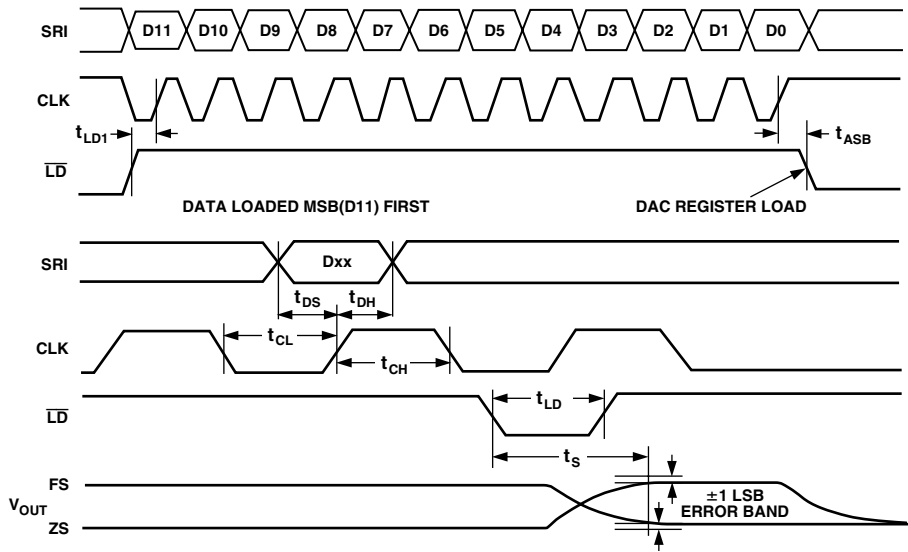
Figure 2. Timing Diagram
