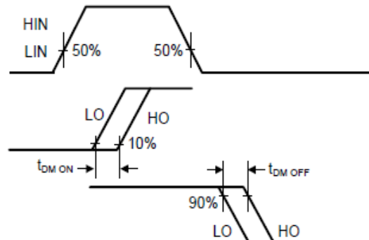
Figure 2. Delay Matching Waveform Definitions
