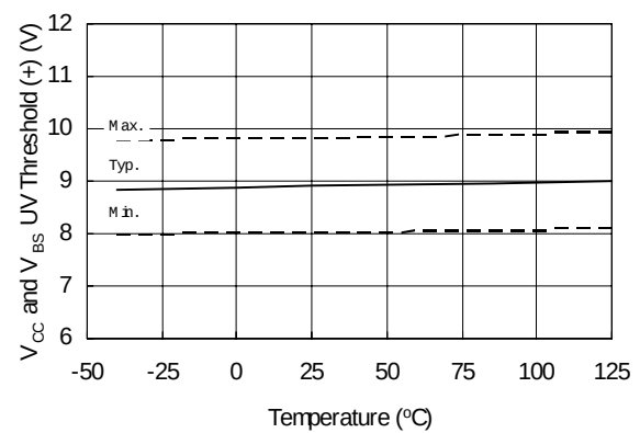
Figure 21. V_{CC} and V_{BS} Undervoltage Threshold (+) vs. Temperature
