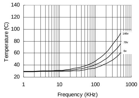
Figure 23. IR2181 vs. Frequency (IRFBC 40), R_{gate}=15\Omega , V_{cc}=15V
